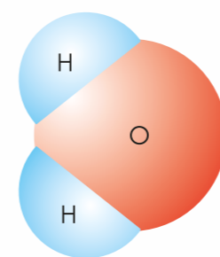
Molecule of water
